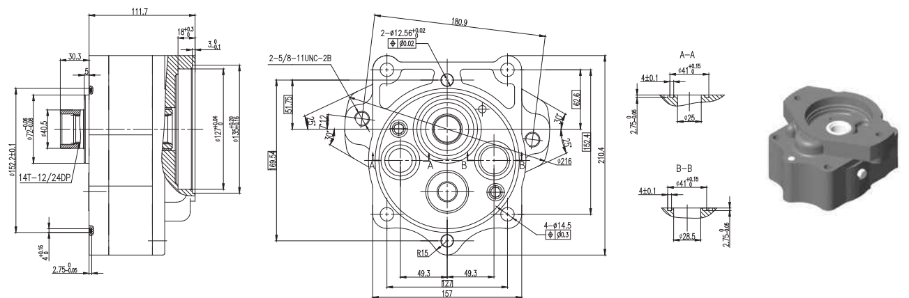
7S4629 Dimensions
