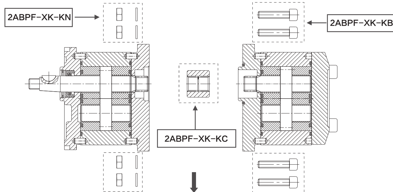
Step 4 Add 2ABPF-XK-K ( Nuts 4 × M10 / Washer 4 × φ 11/ Coupling 1/ Bolt 4 × M10 )
