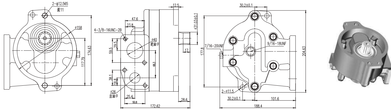
3S4386 Dimensions
