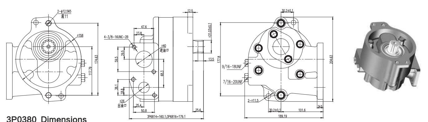
3P0380 Dimensions
